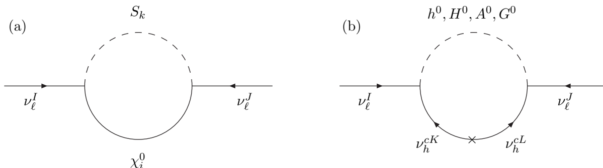
Figure 2: One-loop corrections to light neutrino masses. (a) The loop consisting of light sneutrinos ( S_k , k = 1 \dots 6 ) and neutralinos ( \chi_i^0 , i = 1 \dots 4 ) is the dominant contribution. (b) The loop consisting of a neutral Higgs (or Goldstone) boson and a heavy neutrino contributes a relative correction to the light neutrino mass of at most a few percent. The contributions of the corresponding graphs (not shown) in which the light sneutrinos in (a) are replaced by heavy sneutrinos and the heavy neutrinos in (b) are replaced by light neutrinos are suppressed by an additional powers of \mathcal{O}(vM^{-1}) as explained in D.
