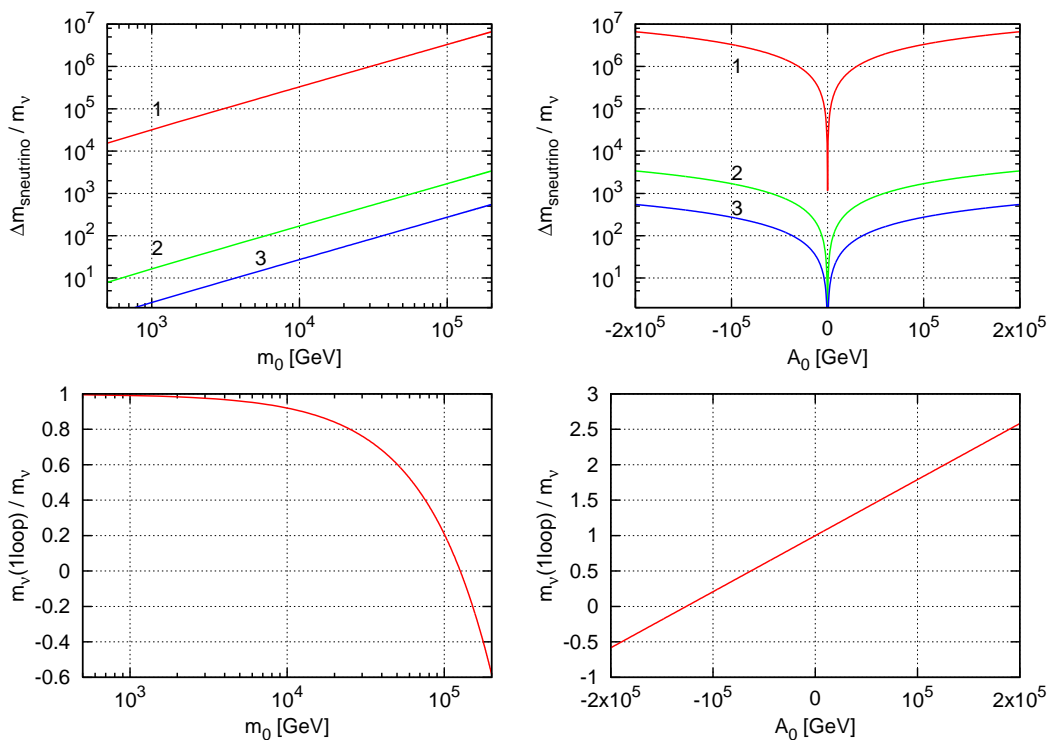
Figure 3: Predictions for the ratios (\Delta m_{\bar{\nu}_\ell} / m_{\nu_\ell})_I and (m_{\nu_\ell}^{(1-loop)} / m_{\nu_\ell})_I for the three neutrino states ( I = 1, 2, 3 ) as functions of the soft SUSY-breaking parameters m_0 and A_0 . When varying m_0 [left panels] we set A_0 = 0 and when varying A_0 [right panels] we set m_0 = 0 .
