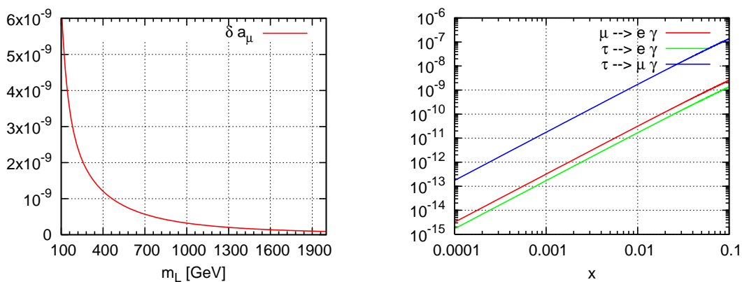
Figure 4: (a) In the left panel, the contribution to the muon anomalous magnetic moment from the diagrams in figure 1 as a function of m_L = m_R is exhibited. (b) In the right panel, the prediction for \text{BR}(\ell^J \rightarrow \ell^I \gamma) is shown as a function of the parameter x = m_N^2 / M^2 . The upper [lower] curves correspond to \tau \rightarrow \mu \gamma [ \tau \rightarrow e \gamma ], and the middle curve to \mu \rightarrow e \gamma .
